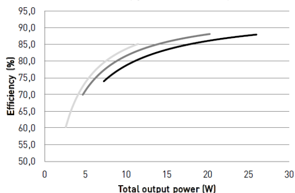
Typical efficiency
