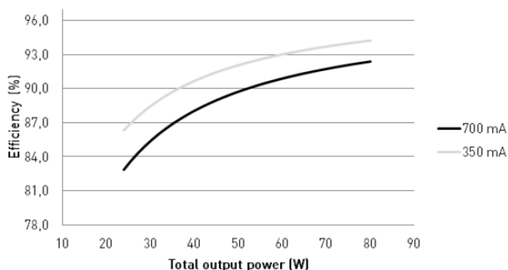
Typical efficiency
